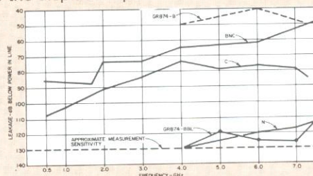
Leakage — note advantage of locking version (874-BBL).
