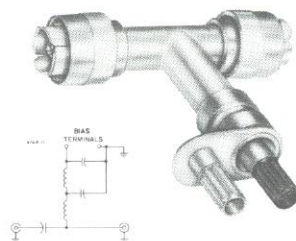
874-FBL Bias Insertion Unit, with locking GR874 connectors
